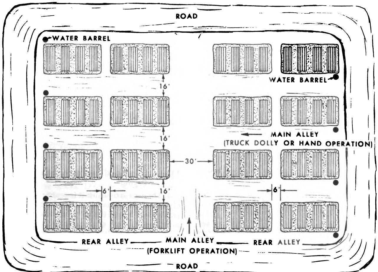
Figure 11-1. A lumberyard layout.
